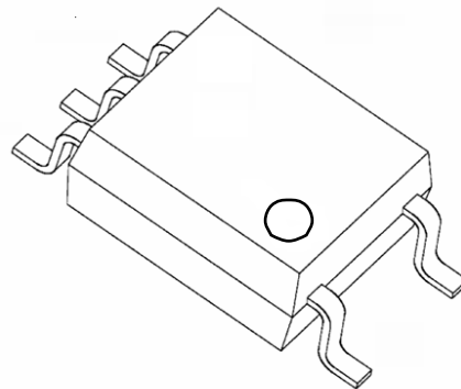
SLM601 SOP-5
